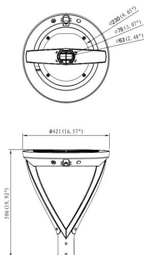
Twin strut mounting
