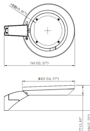
Straight-arm mounting
